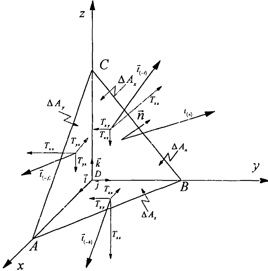
Figure 4 A material volume with surface stresses.
